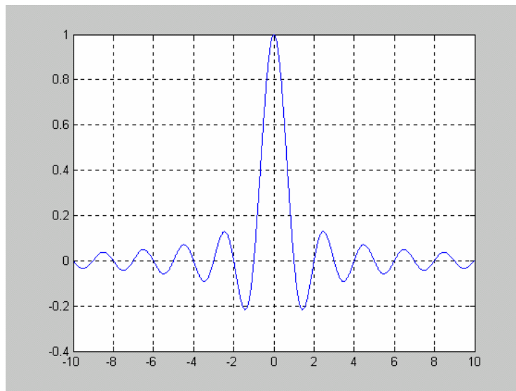
Gambar 1.1. Kurva y=\text{sinc}(x)
